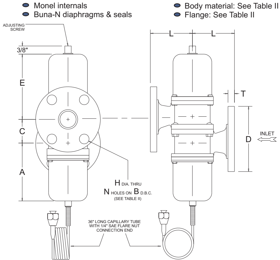
Reference Metrex drawing M900P-FL-2W
